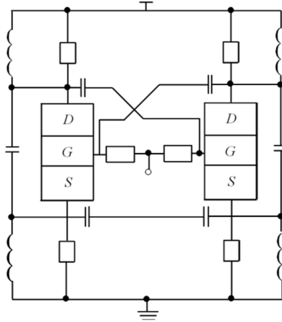
Fig 1a. Structure of the considered oscillator (Roy et al., 2015)
